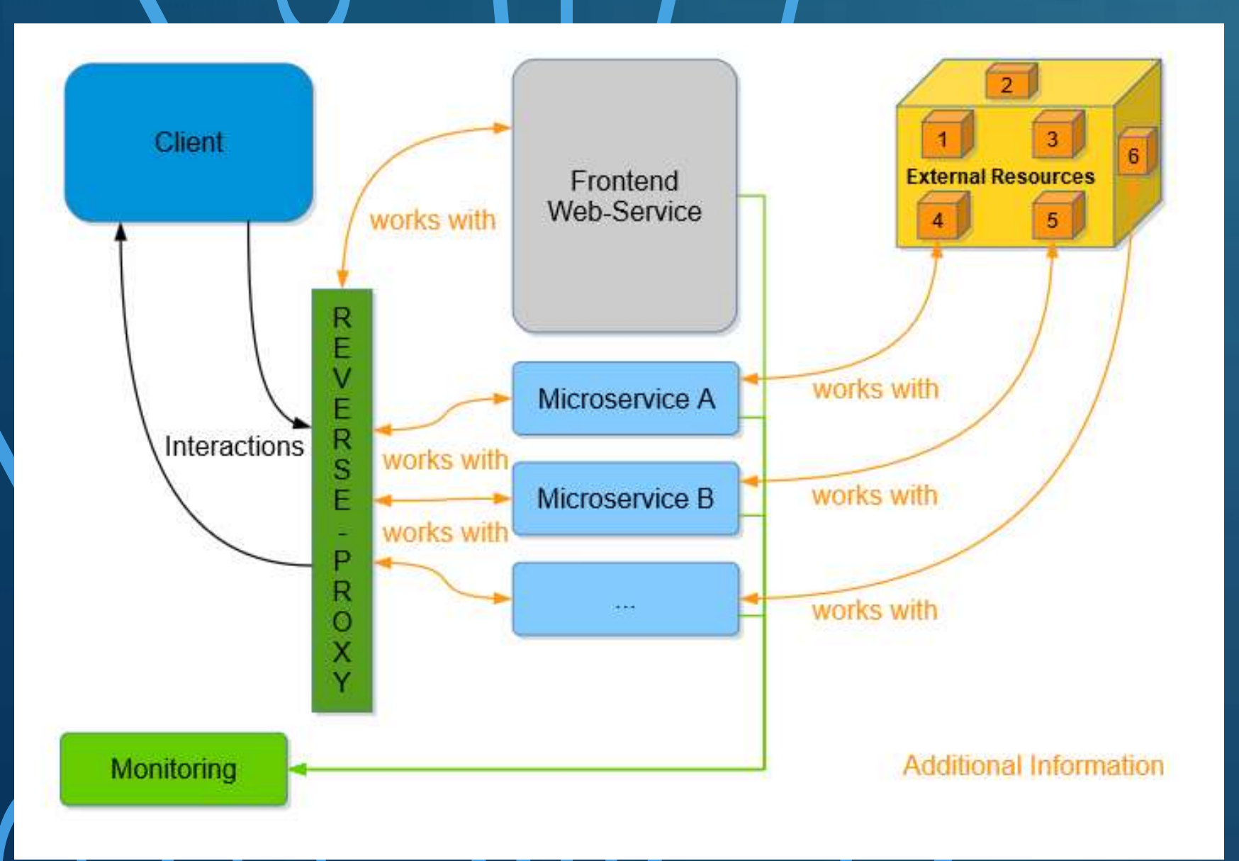
Overview of SlideWiki Microservice Architecture (by Roy Meissner)
